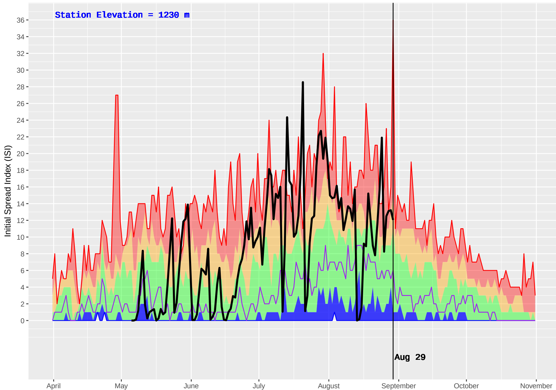
SLOCAN (406) : Historical (1992–2016) and Current (2017) Noon Initial Spread Index (ISI)
