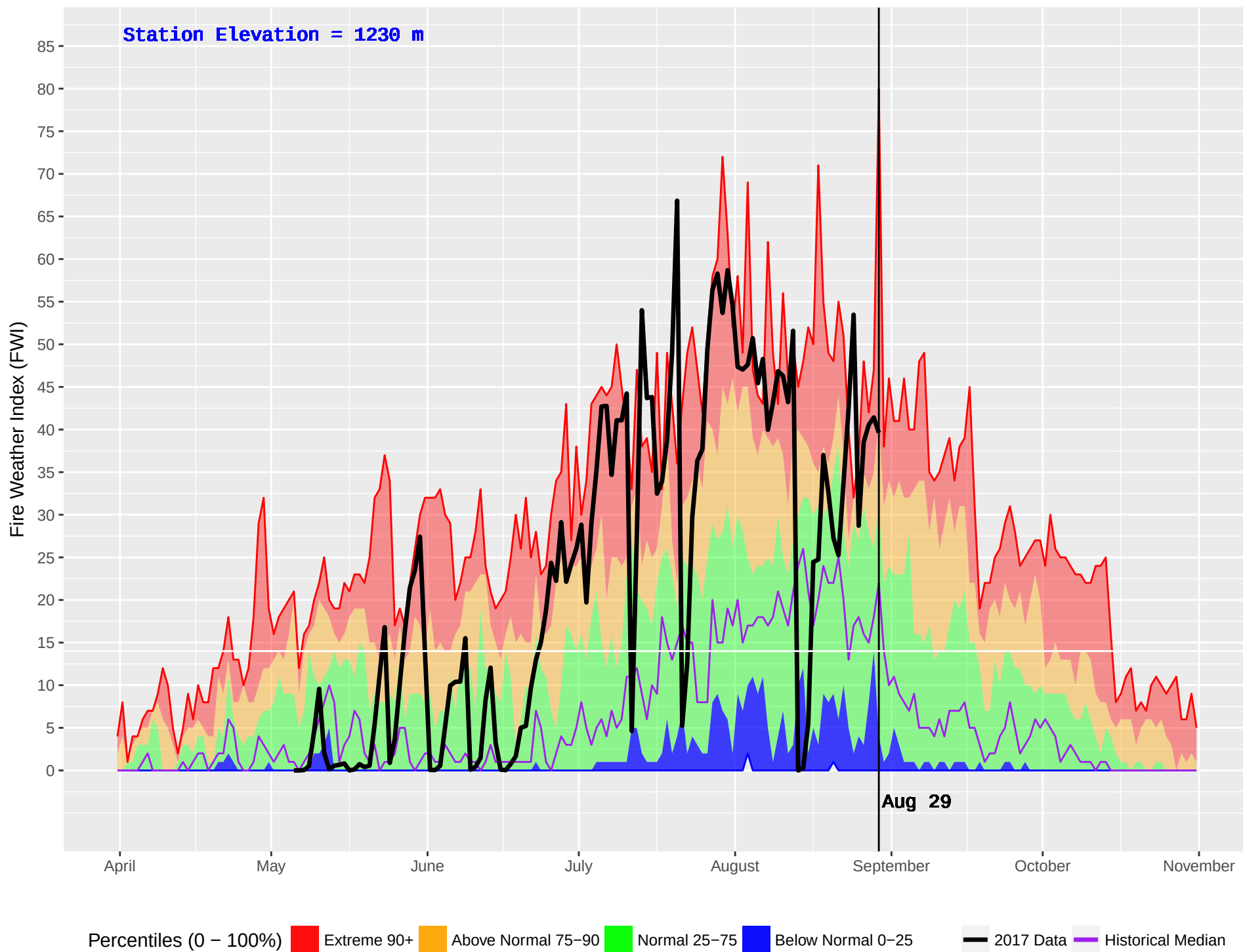
SLOCAN (406) : Historical (1992–2016) and Current (2017) Noon Fire Weather Index (FWI)
