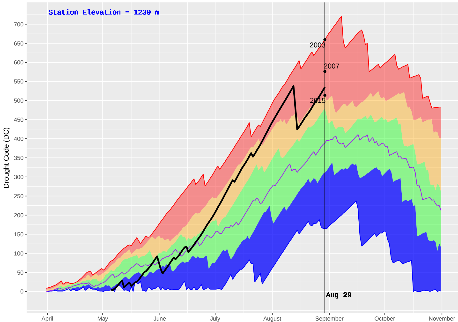
SLOCAN (406) : Historical (1992–2016) and Current (2017) Noon Drought Code (DC)
